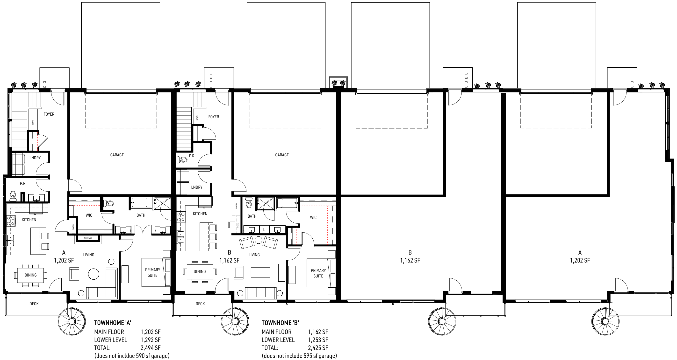
1 FLOOR PLAN - LEVEL 1 3/32" = 1'-0"
